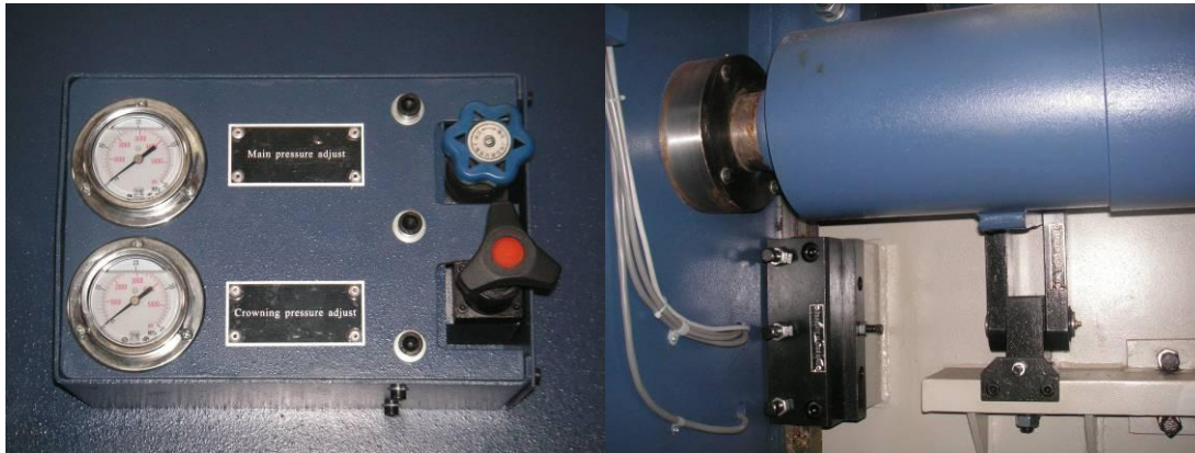
Crowning and main pressure adjustment 200T mechanical balance torsion bar
