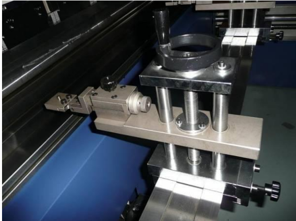
Backgauge with manual R axis
