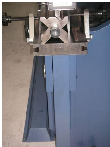
Three plate bottom crowning design
